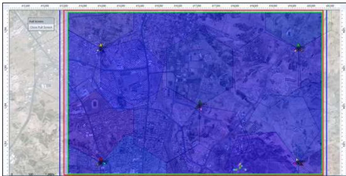
Figure 4. 42: prediction result of Coverage by Quality Indicator (UL) in LTE technology (After optimization)
