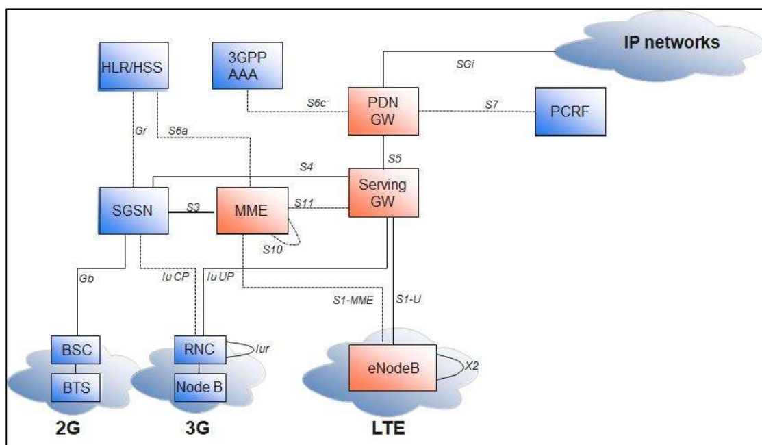
Figure 2. 28: Evolution of LTE
