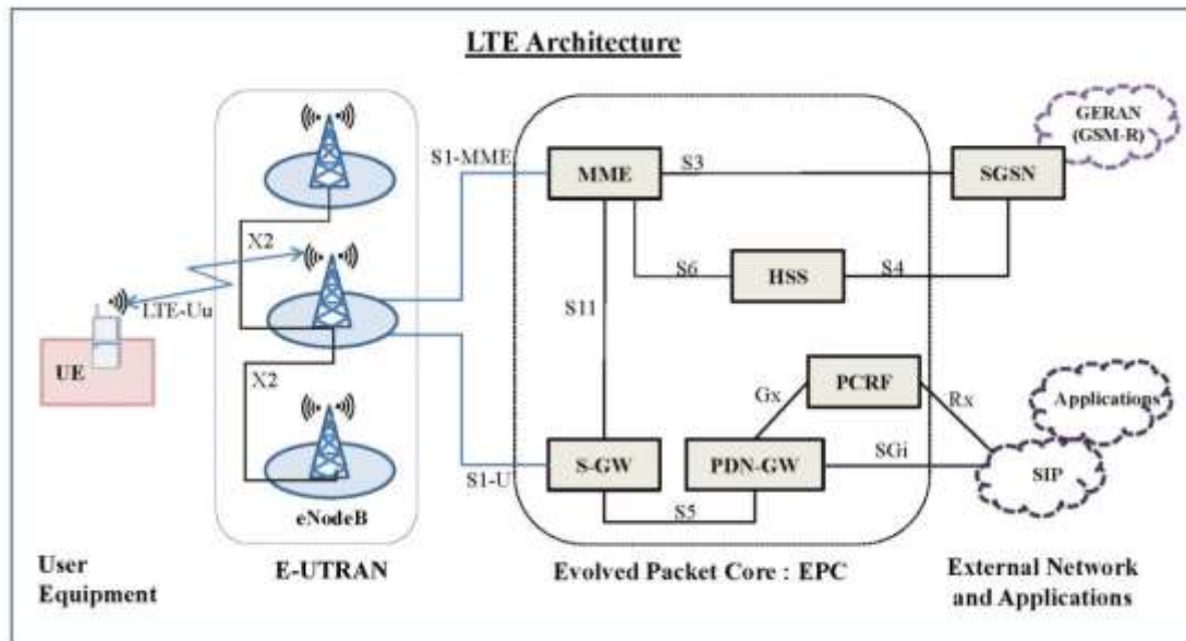
Figure 2. 17: LTE Architecture
