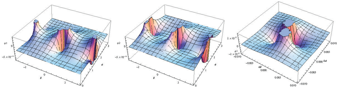
Fig. 3 The left graph shows the 3D plot of \alpha_1 and the middle one shows that of \alpha_2 . Notice that the two graphs are all plotted in the limitation where \{\theta, \phi\} is not close to \{0, \pi/2\} . The right one illustrate the value of \bar{\alpha} when \{\theta, \phi\} \rightarrow \{0, \pi/2\} , where \{\theta, \phi\} \equiv \{\Delta\theta, \pi/2 + \Delta\phi\} .
