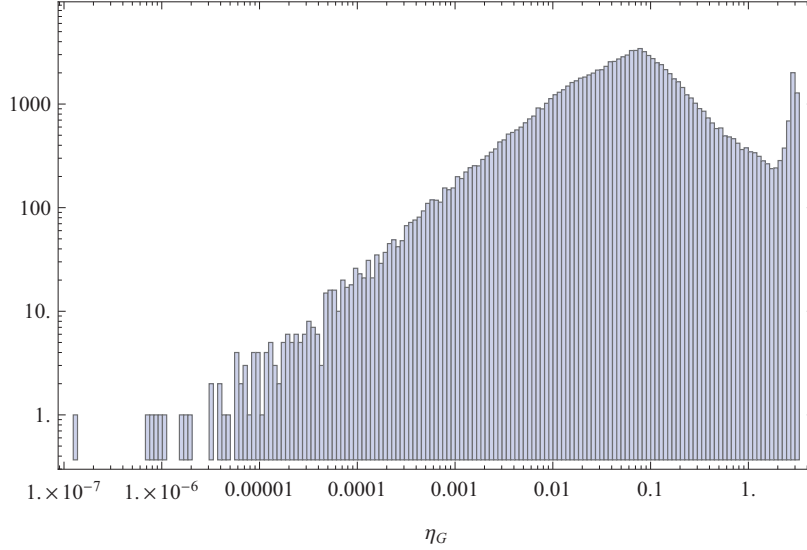
Fig. 5 The distribution of \eta_G is illustrated by this graph in which log-log coordinates make the graph more appropriate. There are about 100,000 points for statistics.
