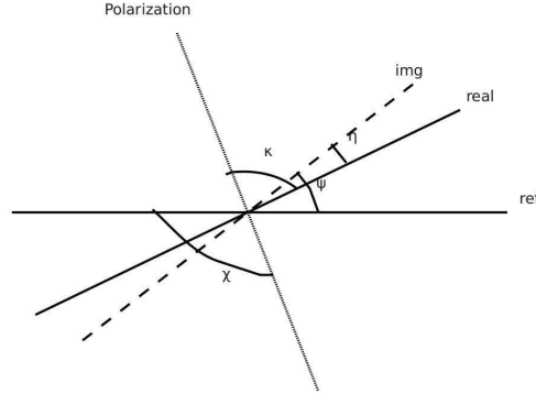
Fig. 1 The relation of the alignment-breaking parameter, \eta_G , to other angles \kappa , \psi , \chi_0 . The dotted (dashed) line represents polarization (image), which is the projection of the direction of polarization on the image plane .
