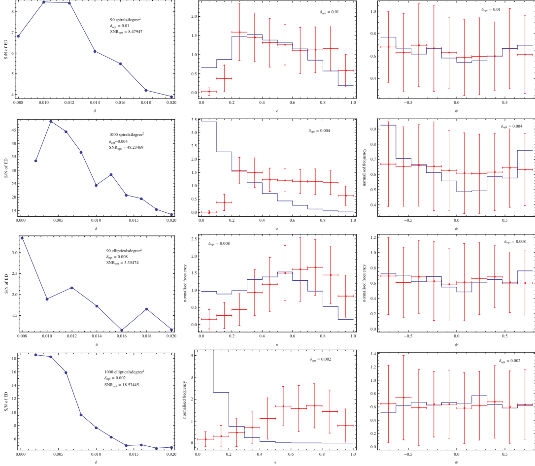
Fig. 6 Left panels show SNRs in the first bin as functions of \delta for different surface number densities and different EDs. Middle and right panels show histograms of lensed EDs and EADs with \delta_{opt} . Each \delta_{opt} is given by the left corresponding graph. The error bars in the first and the third (the second and the fourth) histograms are generated by choosing the point with its parameters obeying the above distributions about n = 90 \Delta\theta^2 180^2 / \pi^2 ( n = 1000 \Delta\theta^2 / \pi ) times and repeating this procedure 100 times. The spirals and ellipticals are created through 100 \times n random choices of \Delta\theta, \Delta\phi \in [-0.5\delta, 0.5\delta] and \{\zeta, \xi\} according to the ellipticity distributions by Padilla and Straus [38], and randomly choosing the points on a unit sphere which gives the distributions of \alpha, \beta, \gamma .
