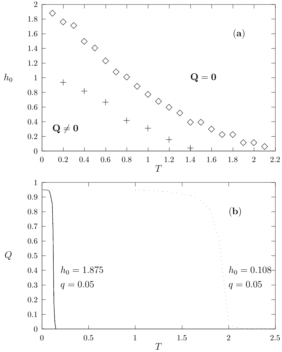
Fig. 2. (a) Projections of dynamic phase surface on the h_0 - T plane. ( \diamond ) represents q = 0.05 and ( + ) represents q = 0.3 . (b) Temperature variations of dynamic order parameter ( Q ) for two different values of field amplitudes ( h_0 ).
