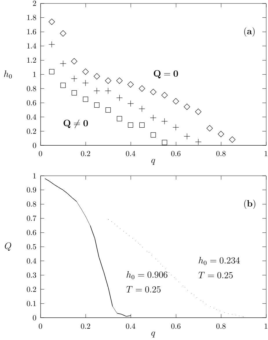
Fig. 3. (a) Projections of dynamic phase surface on the h_0 - q plane. ( \diamond ) represents T = 0.25 , ( + ) represents T = 0.50 and ( \square ) represents T = 0.75 . (b) Variations of dynamic order parameter ( Q ) with respect to impurity concentration ( q ) for two different values of field amplitudes ( h_0 ).
