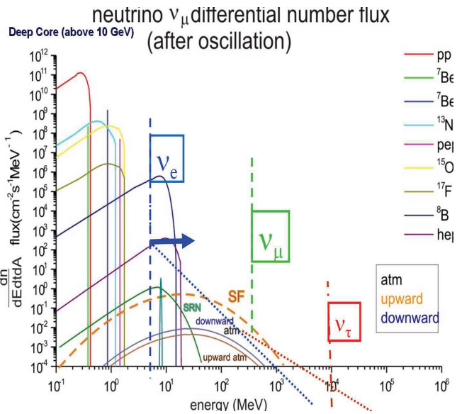
Figure 3: As above, for Deep Core detector above 10 GeV. As shown the \nu_\mu signal is nearly revealed at the GeV edge; however future PINGU enhanced detector might reach the threshold of GeV neutrino discover from solar flare
