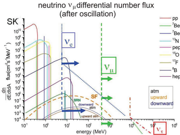
Figure 1: Solar Neutrino \nu_e, \nu_\mu flare versus noises. Note the expected windows by up-down arrows.
