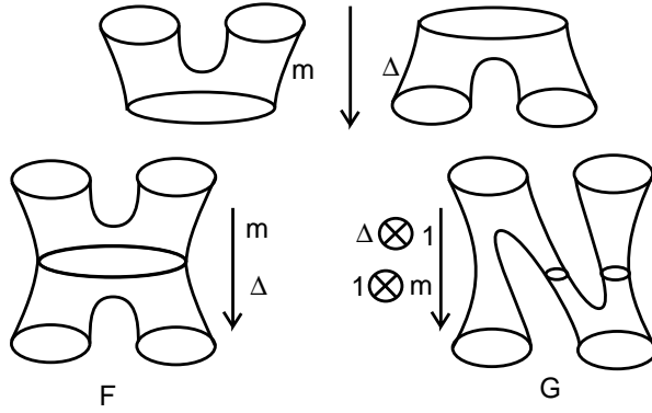
Figure 5: Surface Cobordisms
