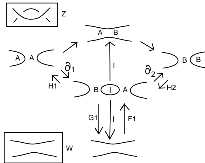
Figure 10: Complexes for Second Reidemeister Move
