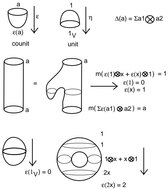
Figure 7: Unit and Counit as Cobordisms
