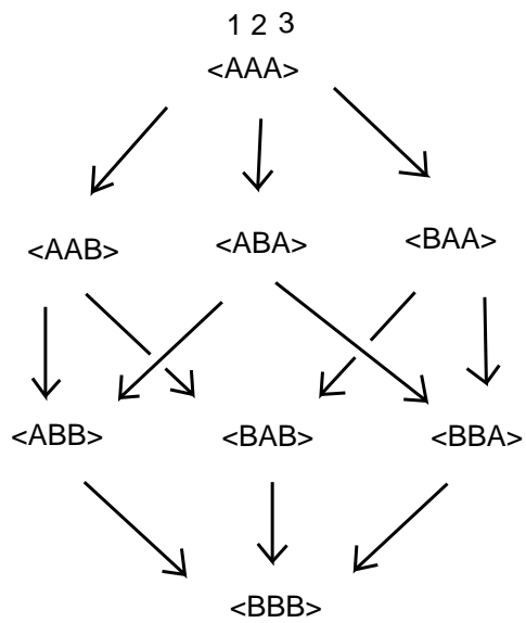
Figure 3: Cube Category
