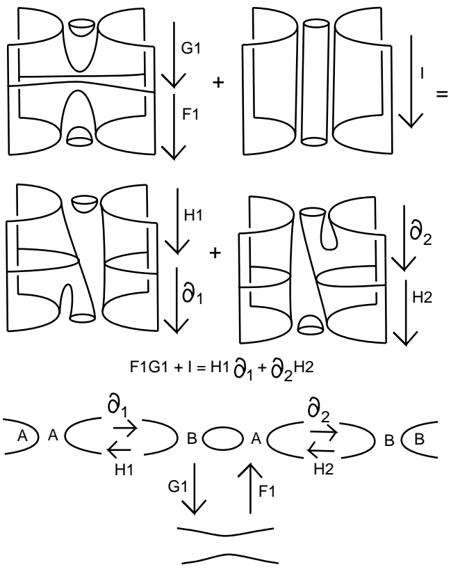
Figure 11: Homotopy for Second Reidemeister Move
