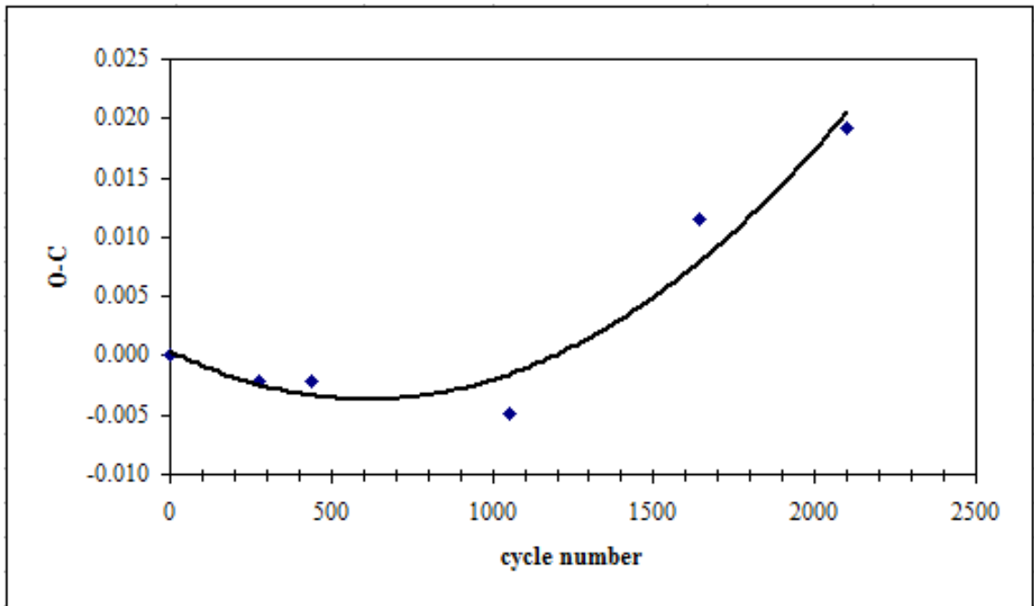
Figure 5. O-C diagram.
