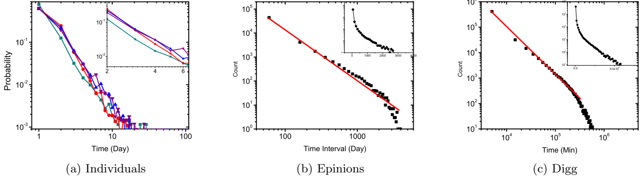
Figure 3: Density plot of waiting times between two consecutive comments from a user, (a) time intervals of four typical users on Digg, (b) intervals from all users in Epinions dataset and (c) intervals from all users in Digg dataset. The upper right plot in (a) shows a zoomed-in view of density plot. The red straight line in (b) and (c) suggests a power-law family of distribution. The plot on the upper right corner in (b) and (c) demonstrates data in a semi-log scale.
